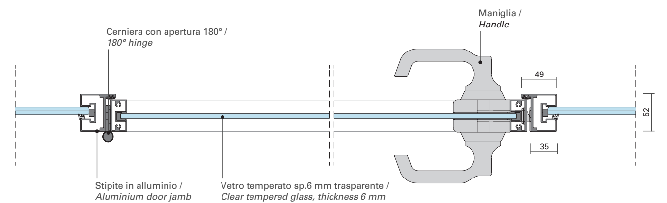
PORTA BATTENTE VETRATA INTELAIATA MINIMAL / MINIMAL FRAMED SWING GLAZED DOOR
