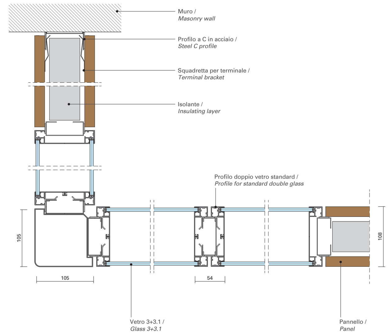
ANGOLO 2 VIE 90° / 2-WAY 90° CORNER PIECE
